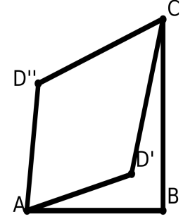
Figure T3 Refuting a SSSSA conjecture
