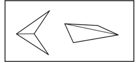
Figure -1 Triangulation of quadrilaterals
