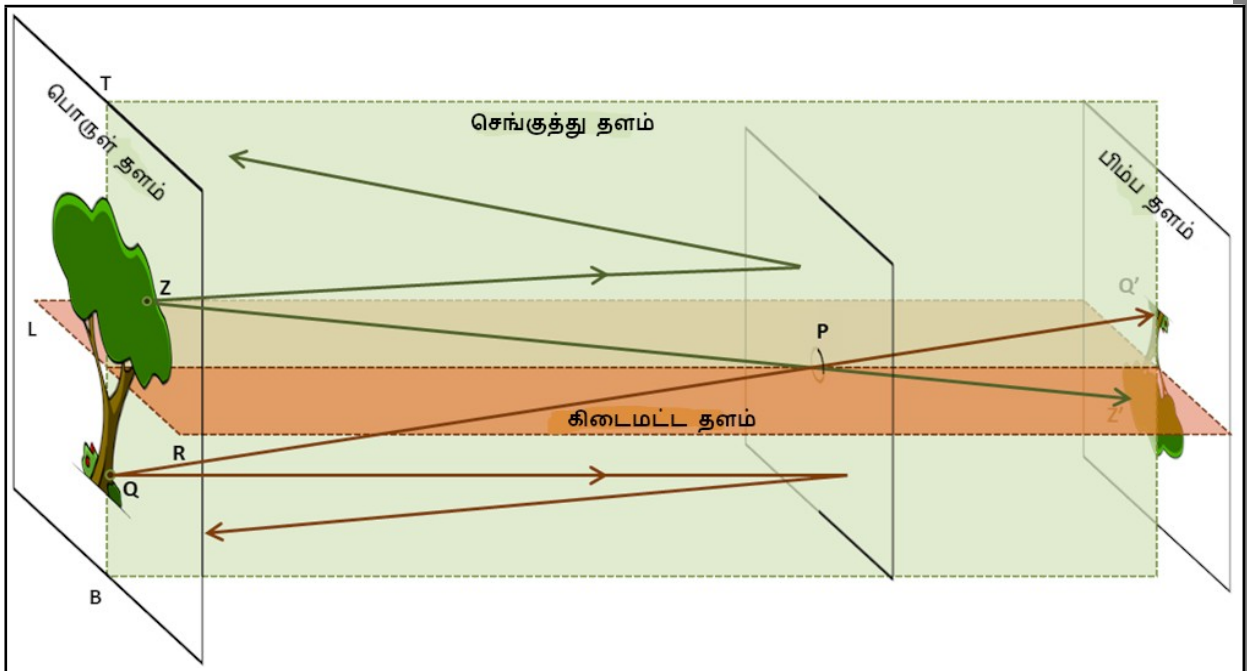
Figure 8T: Ray diagram that can help predict location of various colour points on the screen.
